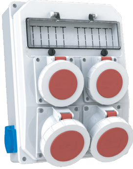
351.5631.5321.222 2(5x63A) CEE IP67/ 2(5x32A) CEE IP67 2(1x16A) Schuko IP54
